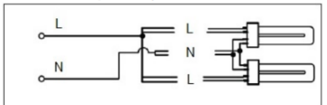
LED PL G24q - 2 lamps
