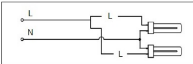
LED PL G24d - 2 lamps
