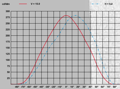
ACT-AS Fluo 2x42W FSM
